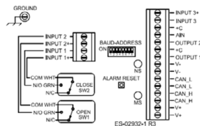
DeviceNet
