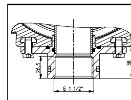
F = Female thread connection
