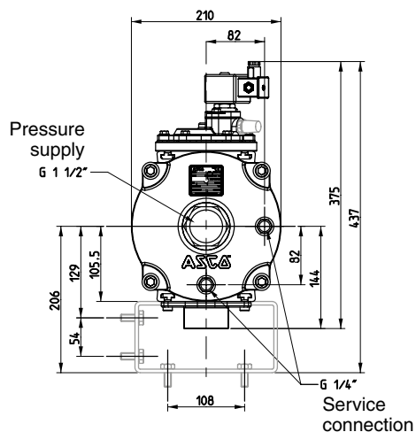
Fig. 1 (front view)
