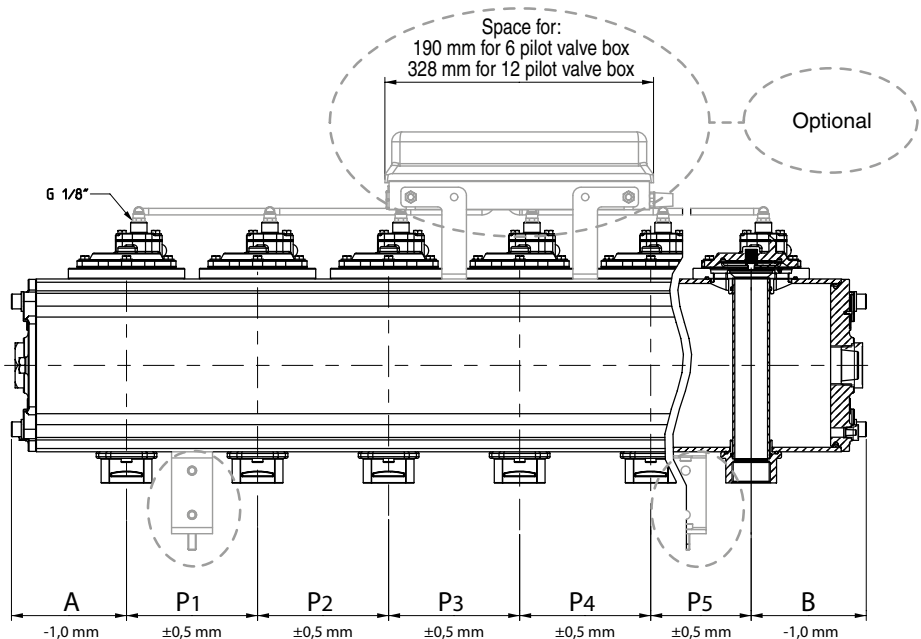
Fig. 2 (side view)
