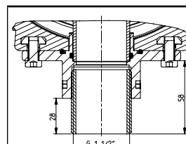
M = Male thread connection
